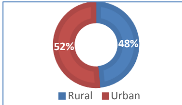
Figure II.1: Population Breakup
